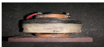
Pinking Coil
